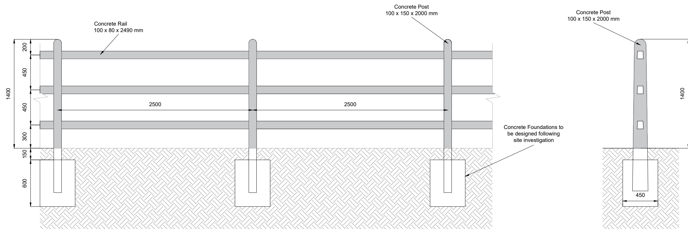
Fence Elevation SCALE 1:30
